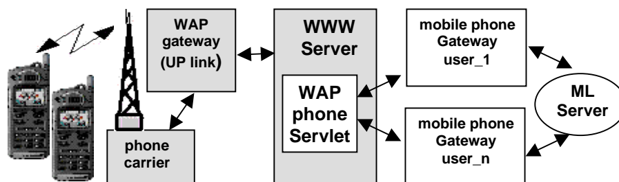
Fig. 6: Refinement of the architecture when relying on WAP. Each mobile is connected the application (running on the ML Server) via a mobile phone gateway A WAP-phone servlet ensures the proper assignments of the devices with their phone gateways.
